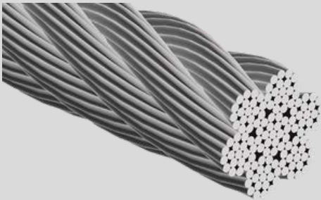
Continuous Wound Cable Construction
