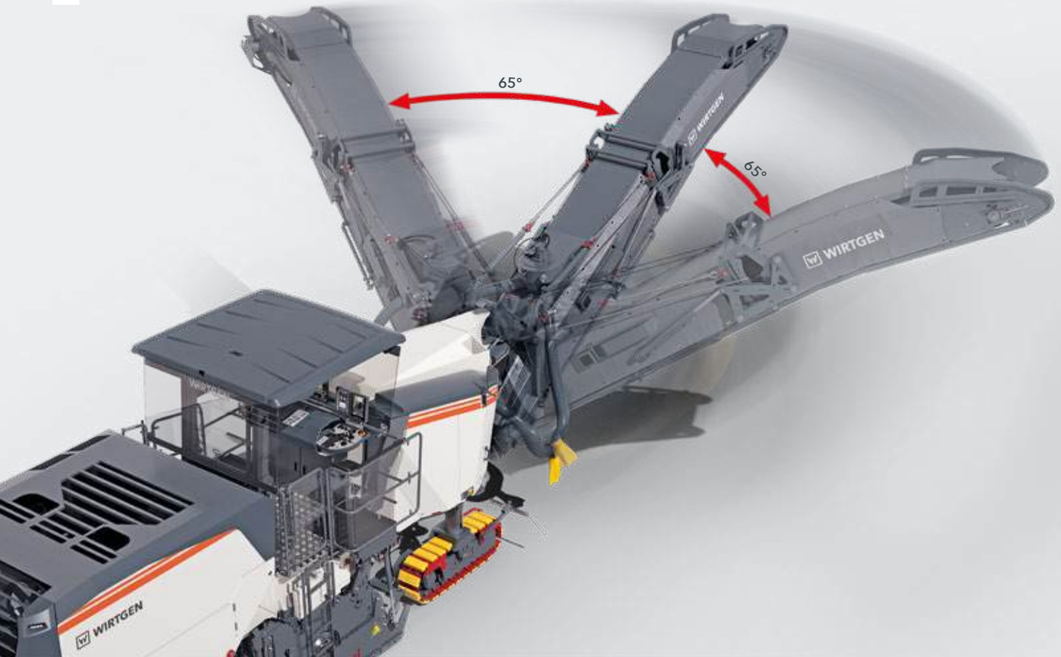
01 Increased scraper lift for a wider range of milling applications and reduced wear. 02 Large discharge conveyor slewing range.
