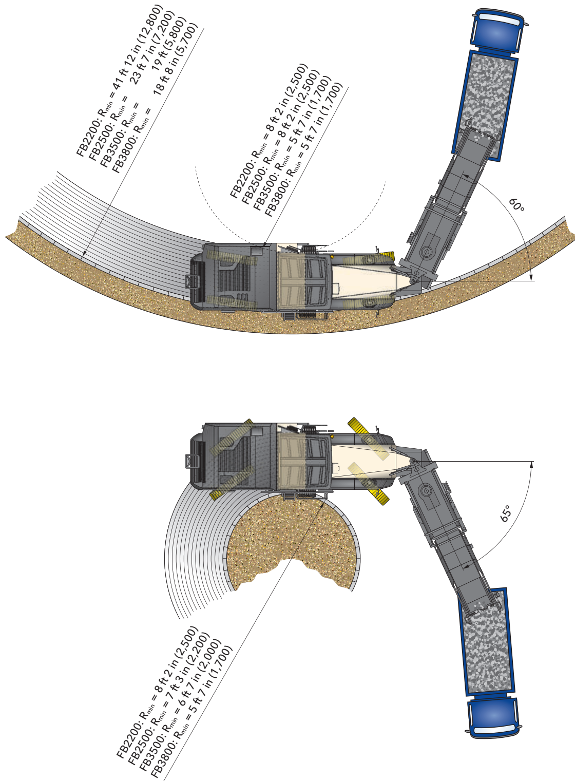
Milling radius at milling depth of 5.9 in (150 mm), dimensions in American standard and mm
