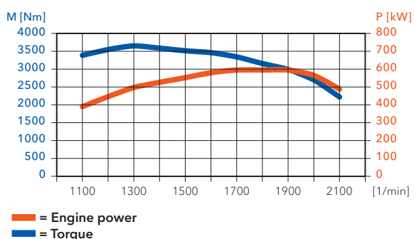
W 220 Fi COLD MILLING MACHINE ENGINE CHARACTERISTICS
