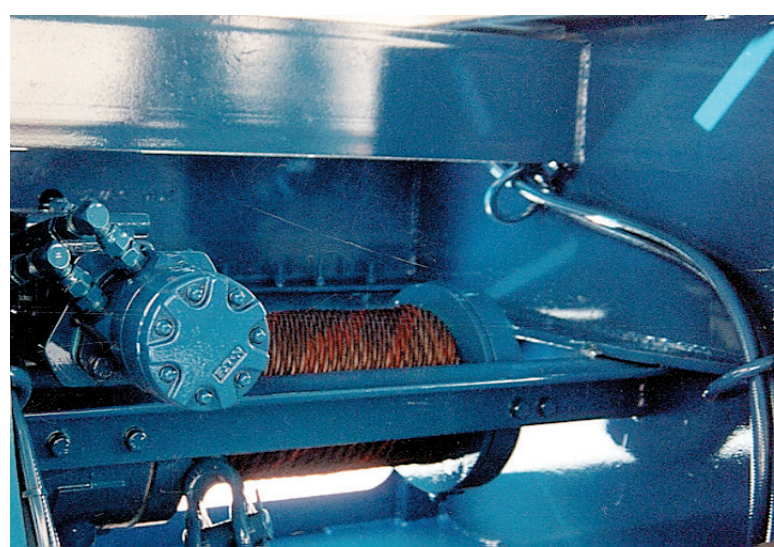
Optional winch built into gooseneck slope.
